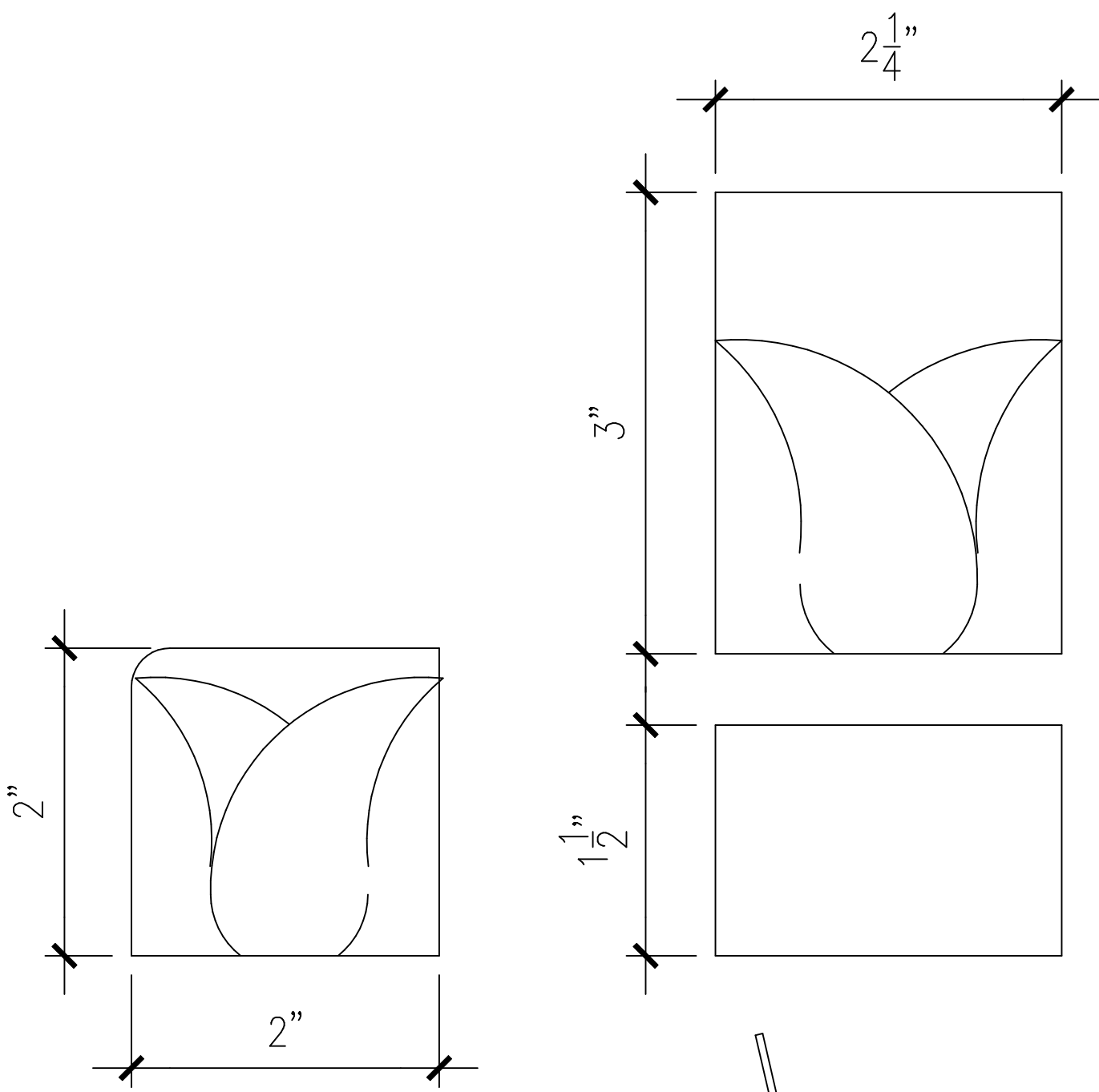
LEFT SIDE (NEED ONE FLIPPED OVER FOR RIGHT SIDE)
